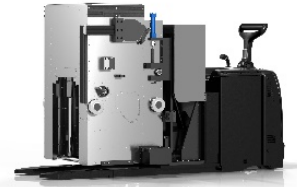
Transport module with Removable Print Module (RPM)
